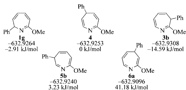
Figure 3. Zero-point-corrected B3LYP/6-31G(d,p) energies (in a.u.) and relative energies for the possible substitution products of benzene by 2c .
