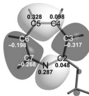
Figure 2. The B3LYP/6-31G(d,p) calculated π LUMO and eigenvectors of the 2p z orbital for the ring atoms of the aromatic methoxyazepinium cation 2c .
