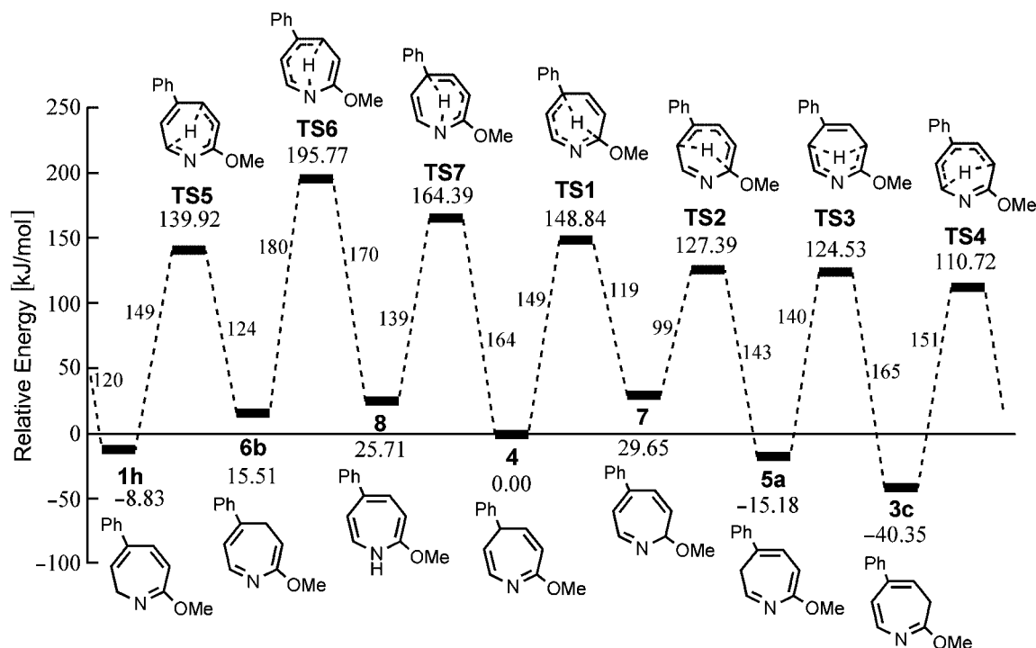
Figure 4. Isomerization pathway of 7-methoxy-4-phenyl-4H-azepine ( 4 ), calculated at the B3LYP/6-31G(d,p) level of theory.
