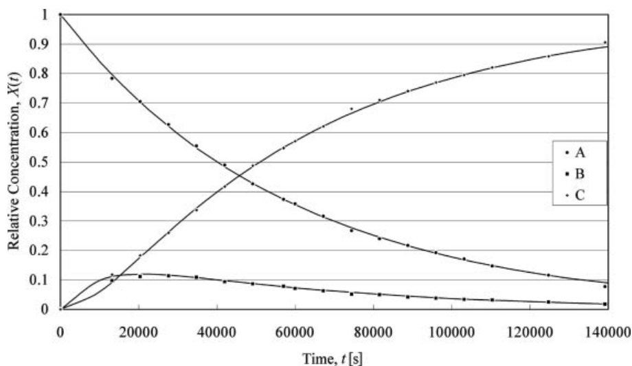
Figure 1. Isomerization of 4 at 162^\circ\text{C} . Points denote A = [ 4 ], B = [ 5a ] and C = [ 3c ] observed by ^1\text{H} NMR spectroscopy. Solid lines represent simulation of two consecutive reactions for k_1 = 1.73 \cdot 10^{-5} and k_3 = 1.00 \cdot 10^{-4} \text{ s}^{-1} .
